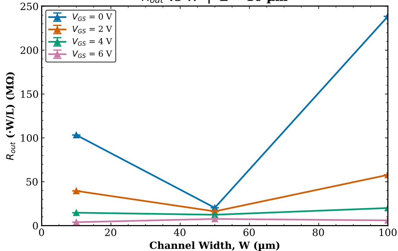
TFT3 Transistor 2 R_{out} vs W | L = 10\text{ }\mu\text{m}
